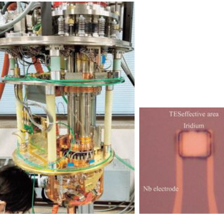
Internal structure of an adiabatic demagnetization refrigerator capable of cooling down to an absolute temperature of 0.05 degrees Kelvin and a superconducting sensor to be installed in the refrigerator. By using this as a detector, we aim to advance radiation measurement technology.
